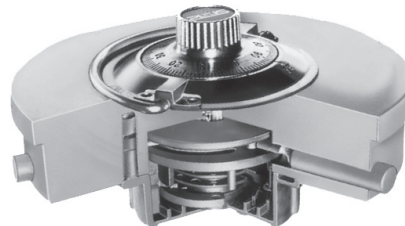
CUTAWAY VIEW “C” RATE LIFT-OUT DOOR
